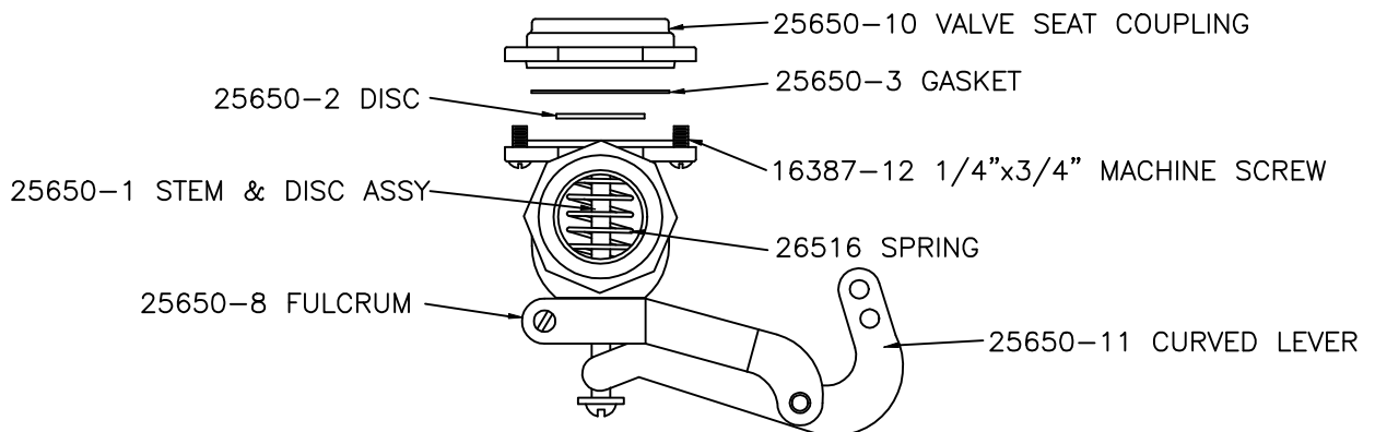
VACUUM VALVE 25650
