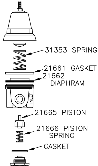
1/4"VARIABLE REGULATOR 31322
