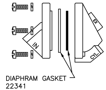
QUICK EXHAUST VALVE 17799
