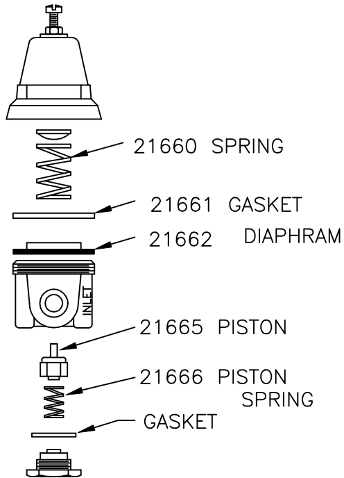
1/4"REGULATOR 16048
